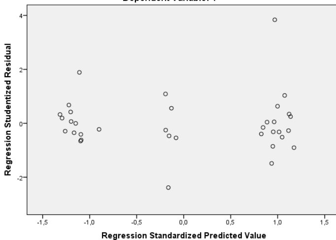
Scatterplot
