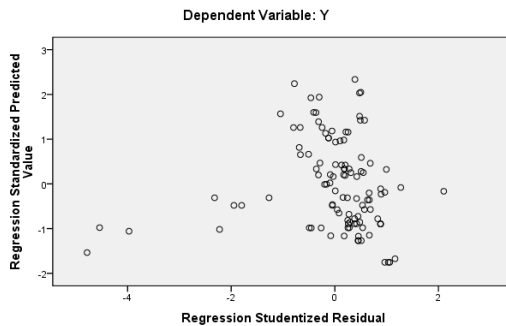
Scatterplot
