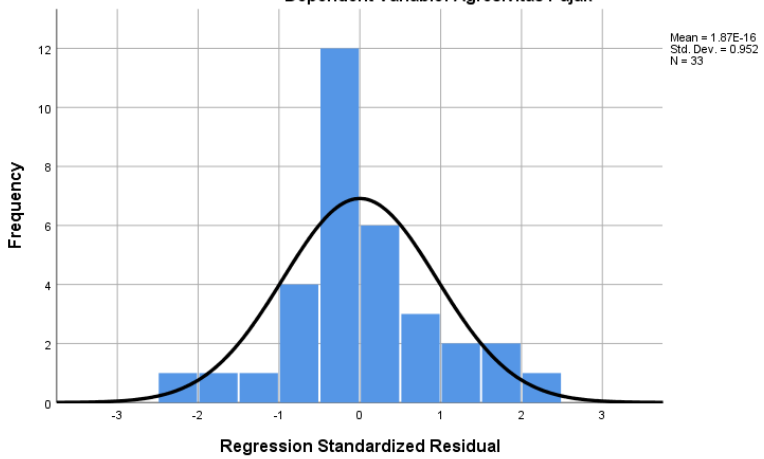
Dependent Variable: Agresivitas Pajak
