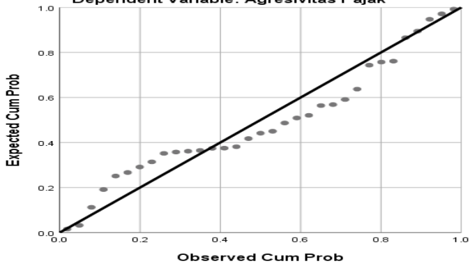
Normal P-P Plot of Regression Standardized Residual Dependent Variable: Agresivitas Pajak
