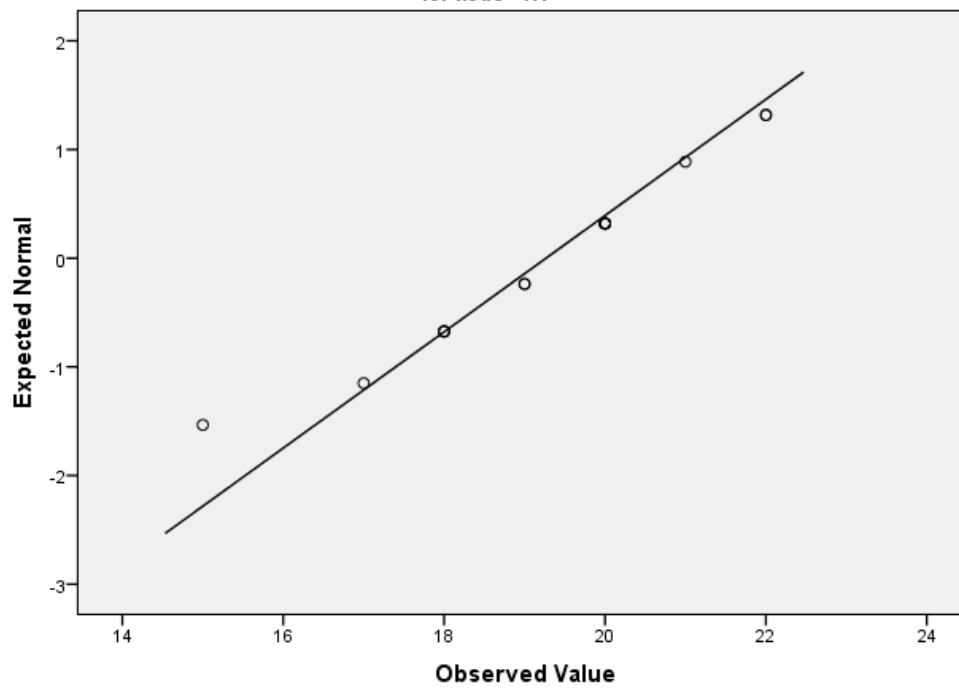
Normal Q-Q Plot of Minyak Kelapa
