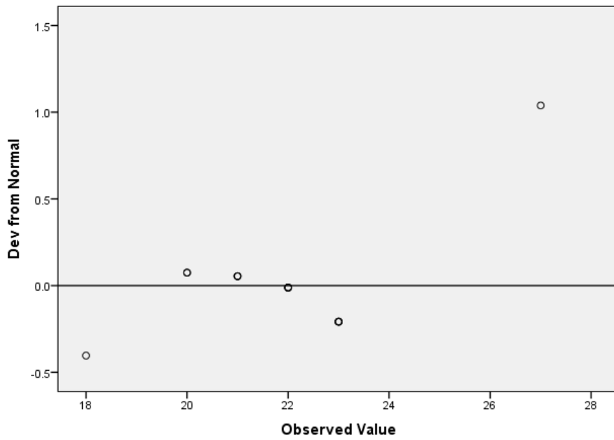
Detrended Normal Q-Q Plot of Minyak Kelapa
